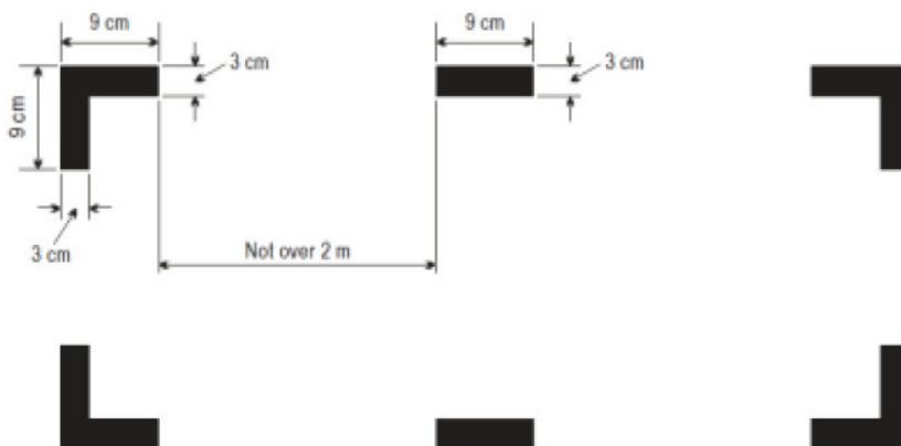
Figure 1. Marking of Break - in Points
